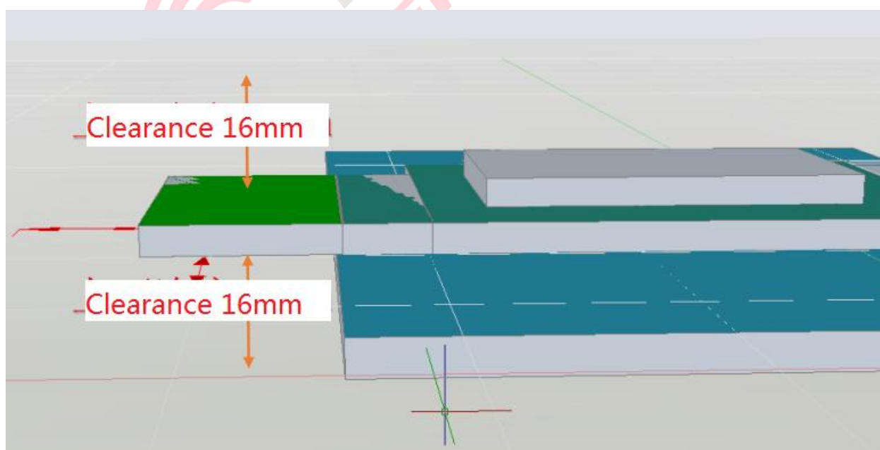
Figure 6-2 Antenna clearance reference
