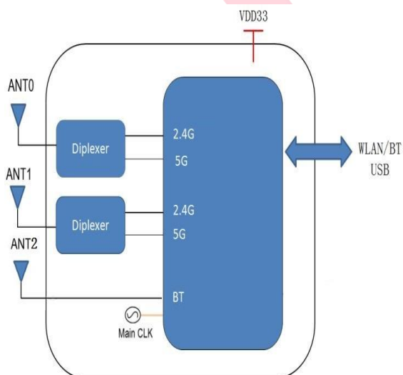
3 Antenna version
