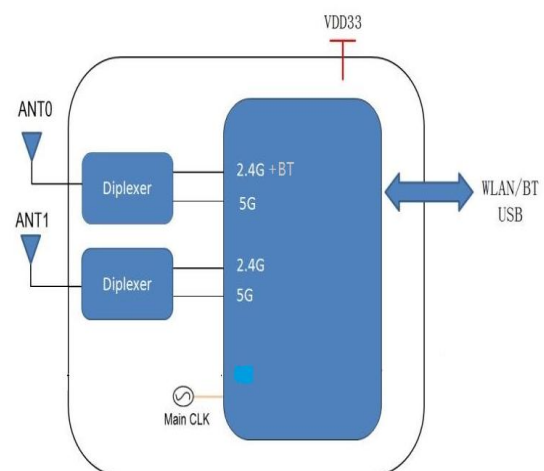
2 Antenna version
