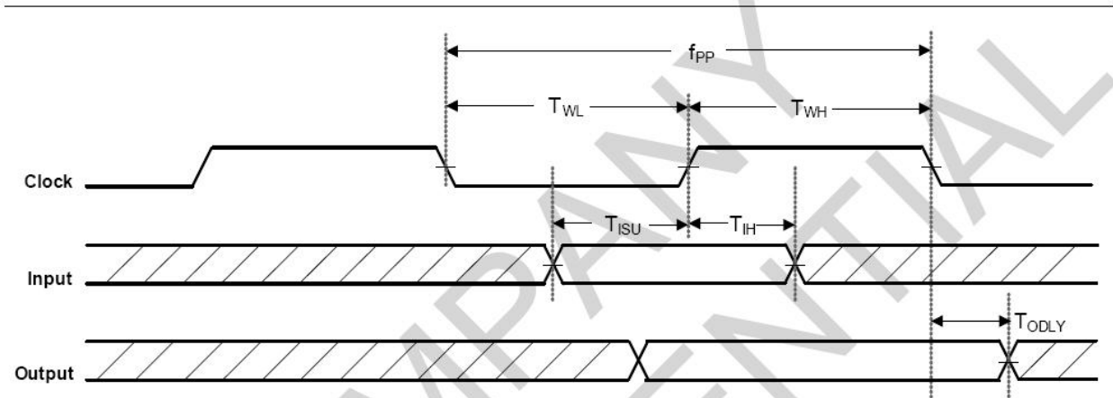
SDIO Protocol Timing Diagram—Default Speed Mode (3.3V)
